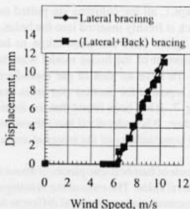
Figure 8 : Effect of back bracing on lateral displacement
