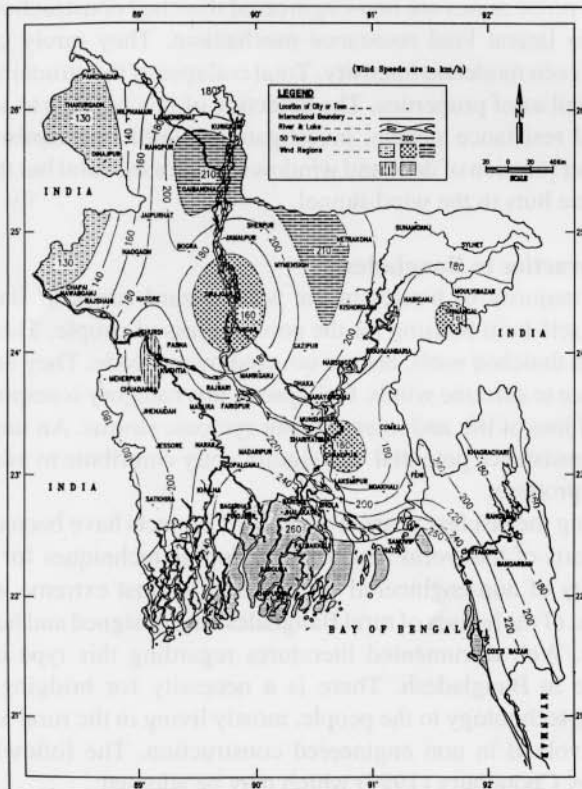
Figure 1 : Basic wind speed map of Bangladesh
