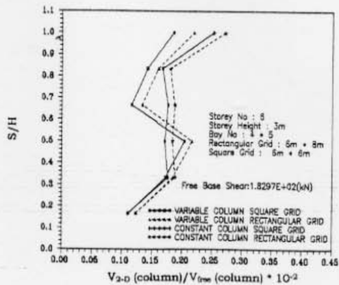
Fig 11. Shear ratio ( V_{2-D}/V_{free} ) versus height ratio ( S/H ) for different column size along height and grid size for 6-storeyed buildings
