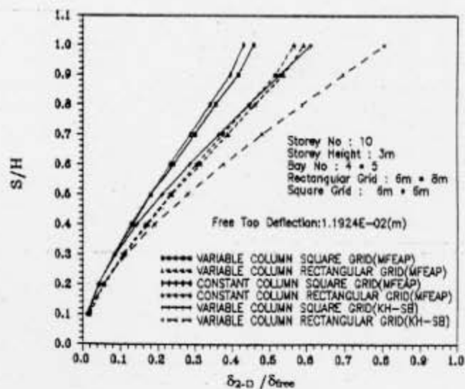
Fig 4. Displacement ratio ( \delta_{2-D} / \delta_{free} ) versus height ratio ( S/H ) for 10-storeyed buildings
