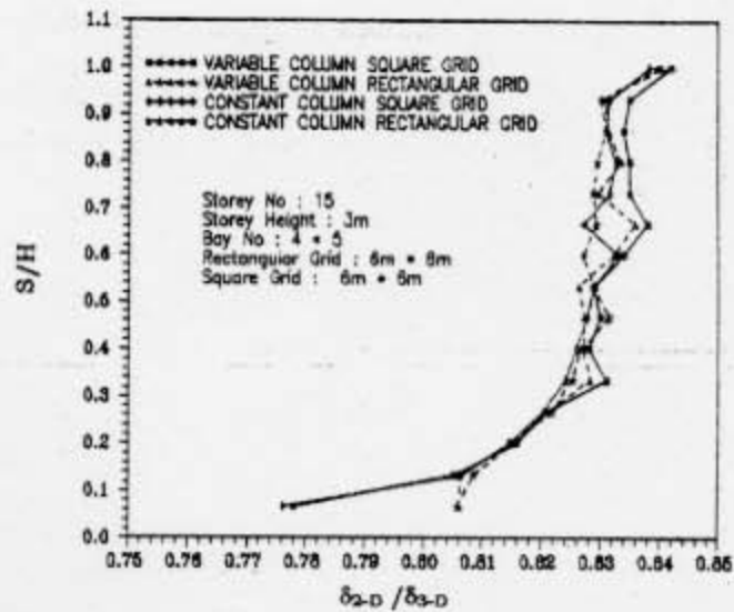
Fig 6. Displacement ratio ( \delta_{2-D} / \delta_{3-D} ) versus height ratio ( S/H ) for 15-storeyed buildings
